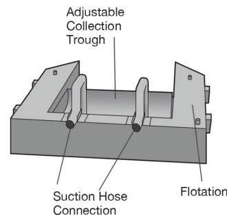
Diagram 5.4.2d Adjustable, Half-Barrel Weir-Type Skimmer
