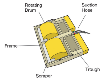
Diagram 5.4.1a Drum Skimmer
