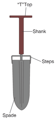
Diagram 5.1.3a Spade Anchor
