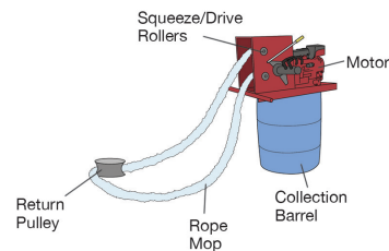
Diagram 5.4.1b Multi-Sided Skimmer
